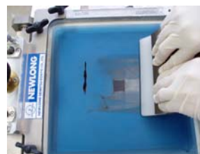
Fig. 3 Process of printing catalyst paste on carbon paper by using hand screen-printing machine
