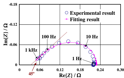
Fig. 12 Nyquist plots of impedance spectrum of the MEA with Electrode-2
