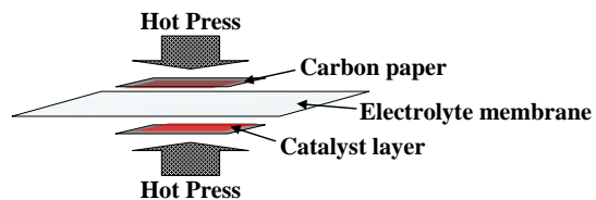
Fig. 5 Fabrication of the MEA by hot pressing carbon paper and electrolyte membrane
