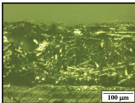
Fig. 11 Cross-sectional optical micrograph of the MEA with Electrode-2
