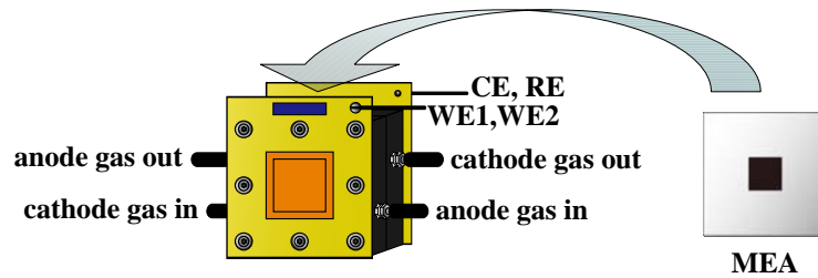
Fig. 6 Single cell for PEFC
