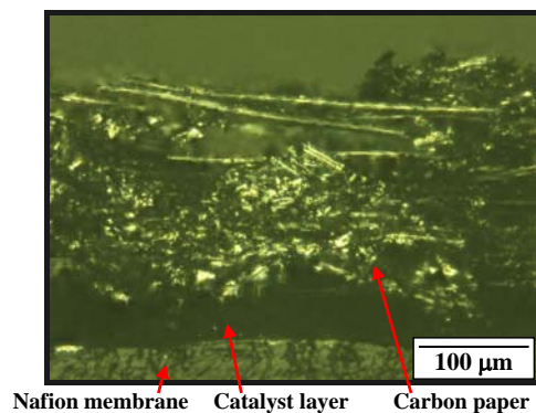
Fig. 9 Cross-sectional optical micrograph of the MEA with Electrode-1
