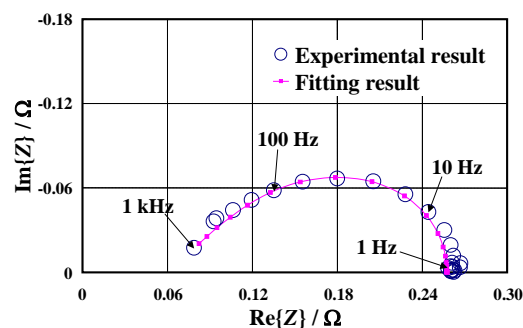
Fig. 10 Nyquist plots of impedance spectrum of the MEA with Electrode-1
