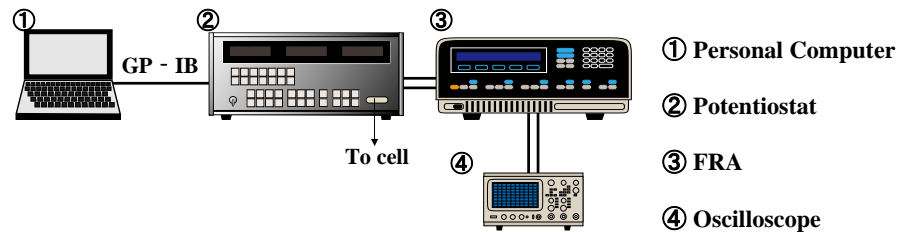
Fig. 7 Schematic diagram of the experimental apparatus
